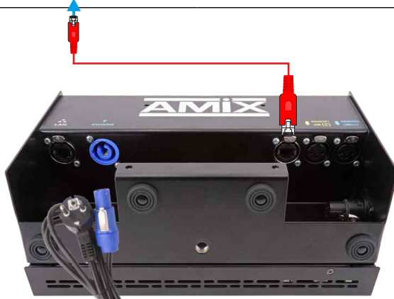
AFF Touring rear panel
